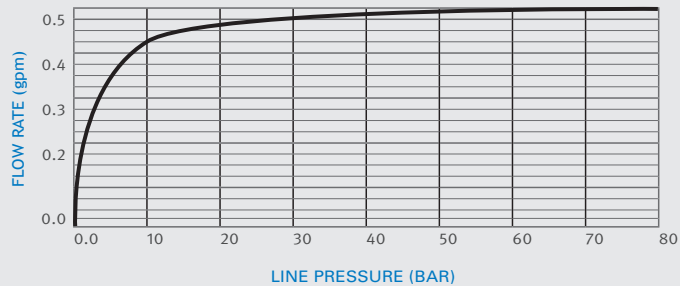
FLOW RATE vs PRESSURE
